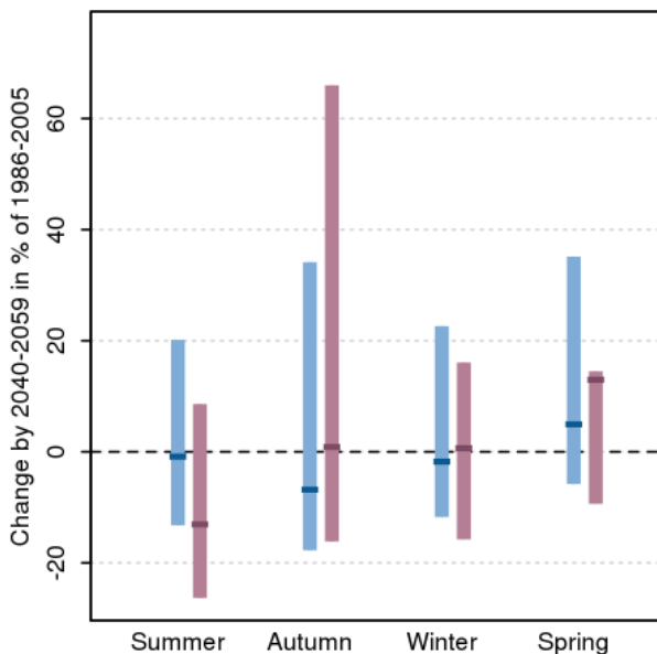
Figure 4. Projected percentage change in the 1-in-20-year maximum daily rainfall for 2040–2059 compared to 1986–2005. Blue bars (left): medium emissions. Purple bars (right): high emissions. Dark horizontal lines: median.
